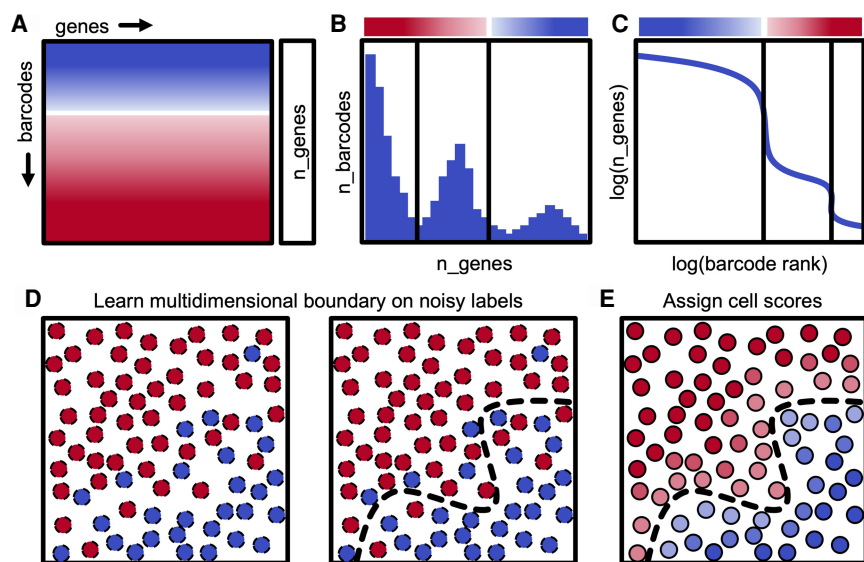
Figure 2. Description of dropkick filtering method. (A) Diagram of scRNA-seq counts matrix with initial cell confidence for each barcode based solely on total genes detected ( n\_genes ), depicted by color (red, empty droplet; blue, real cell). (B) Histogram showing the distribution of barcodes by their n\_genes value. Black lines indicate automated thresholds for training the dropkick model. (C) \log(n\_genes) versus \log(\text{rank}) representation of barcode distribution as in dropkick QC report (Fig. 1A). Thresholds from B are superimposed. (D) Thresholds in heuristic space (B,C) are used to define initial training labels for logistic regression. (E) dropkick chooses an optimal regularization strength through cross-validation and then assigns cell probabilities and labels to all barcodes using the trained model in gene space.
